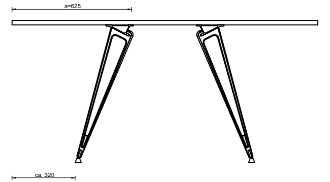
D Innermost acceptable beam placement, according to TGS intuition
