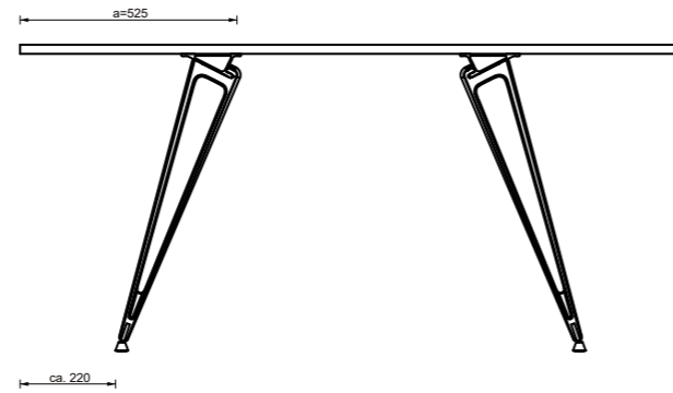
B Beam placement as width 120cm, according to design-manual
