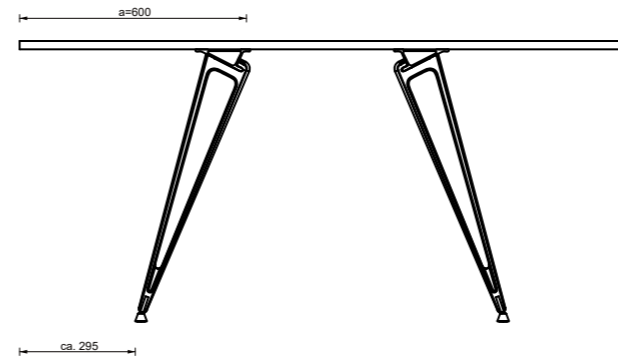
C Variation C
